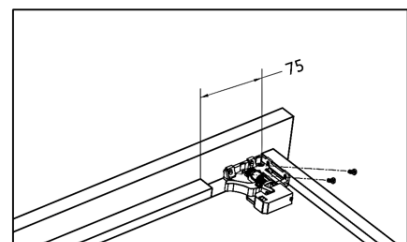
Drawer size and drilling (mm)
