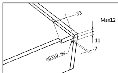
Drawer size and drilling (mm)
