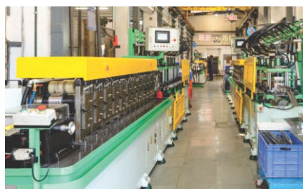
Roll Forming Production Line
