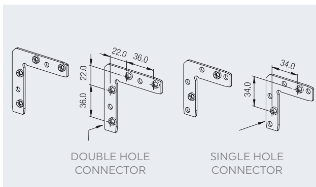
Corner Brackets for Glass Shutter Profile
