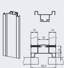
Vertical Gola Profile C
