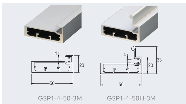
Al. Profile Glass Shutter 50mm
