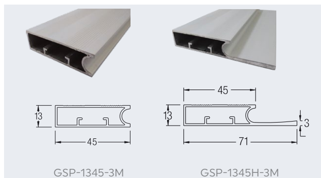
Al. Profile Glass Shutter 1345
