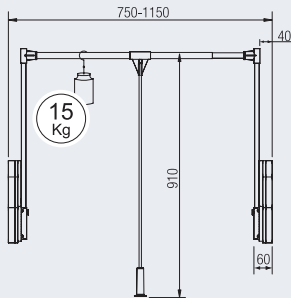
Wardrobe Lift Side Mount-15 Cabinet- Width: 750-1150mm Finish: Grey/Black
