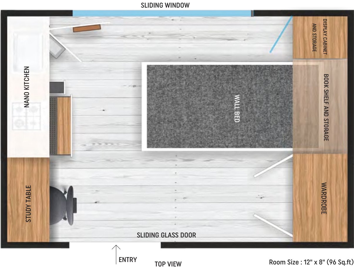
TOP VIEW
