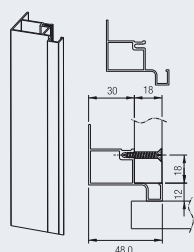
Vertical Gola Profile L
