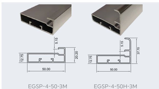
Al. Profile Glass Shutter Euro 50mm
