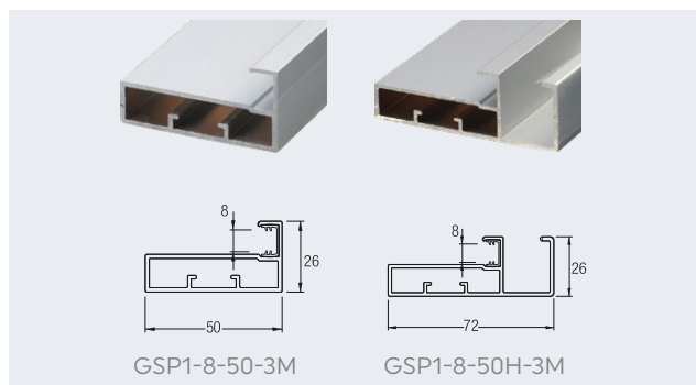
Al. Profile Glass Shutter 8-50mm
