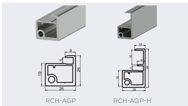
Recessed Hinge Profiles
