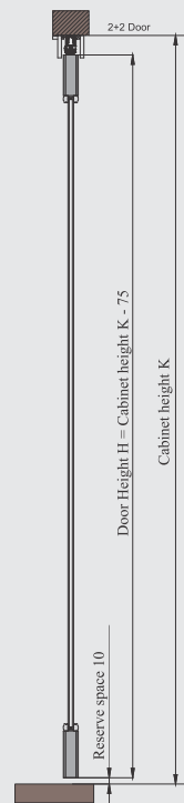
Wooden Door
