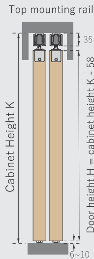
Wooden Door
