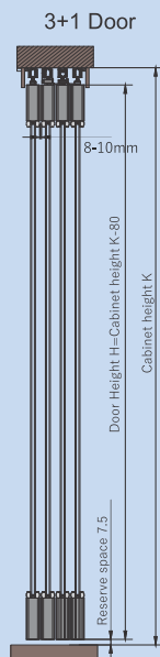
Wooden Door
