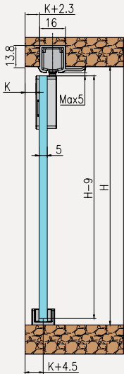
Top Track (Single Door)
