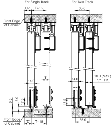
Hi Slide 90 (Soft Close)
