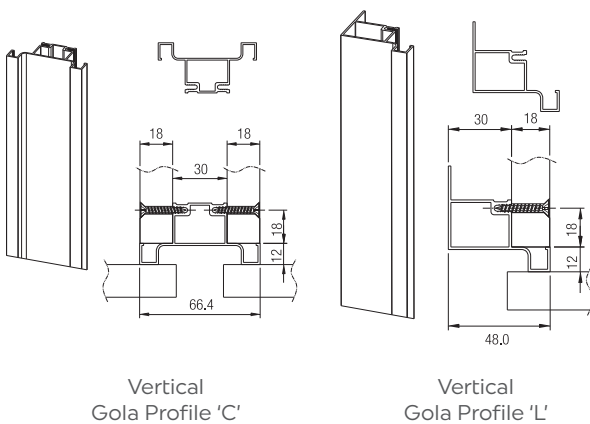
| VERTICAL GOLA PROFILES |
