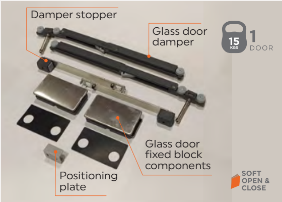
Hi Slide Glass Display 15
