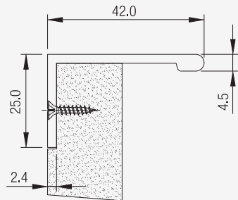
Recessed Handle Steel Furniture.
