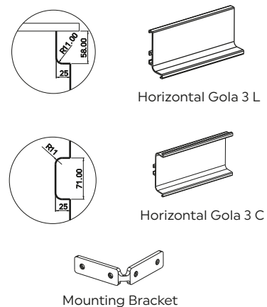
| HORIZONTAL GOLA PROFILES |
