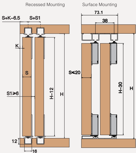
Hi Slide 50 Reversible
