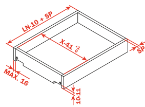
Internal drawer (view from above)
