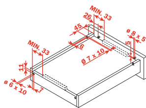
Drawer with frontal (view from below)
