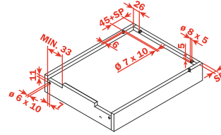
Internal drawer (view from below)
