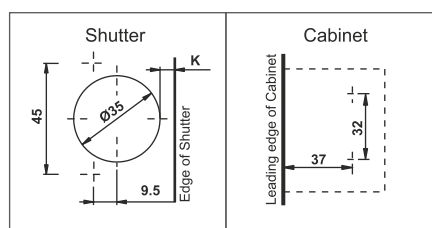
Magnetic Release Device
